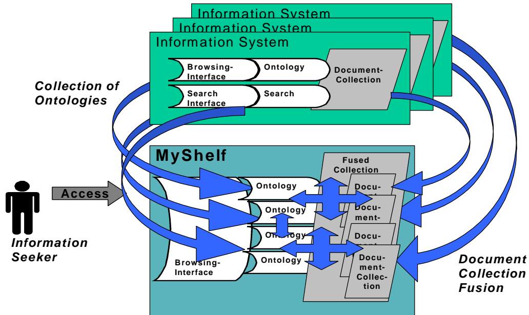
Figure 1: MyShelf as integrated information system
