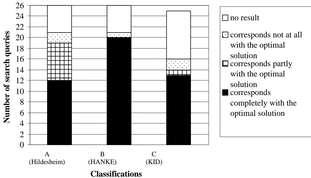
Figure 5: The classifications in comparison
